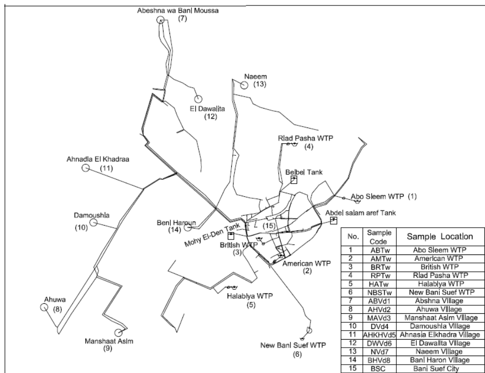
Figure 4. The fifteen sampling points (codes) on the general layout of BSWDN.
