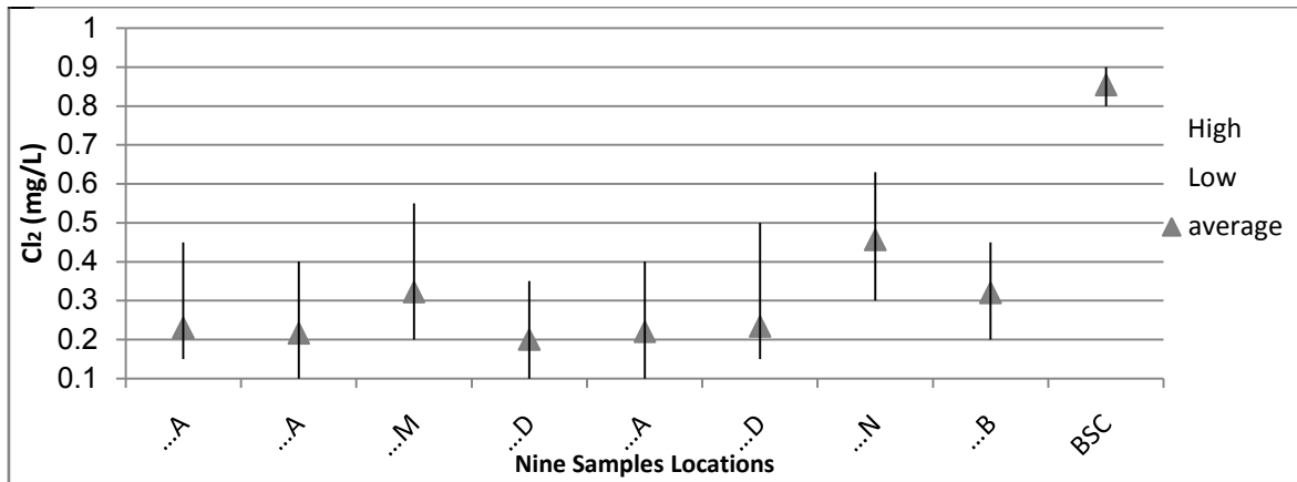
Figure 8. Concentrations of free residual chlorine at the nine points on BSWDN
