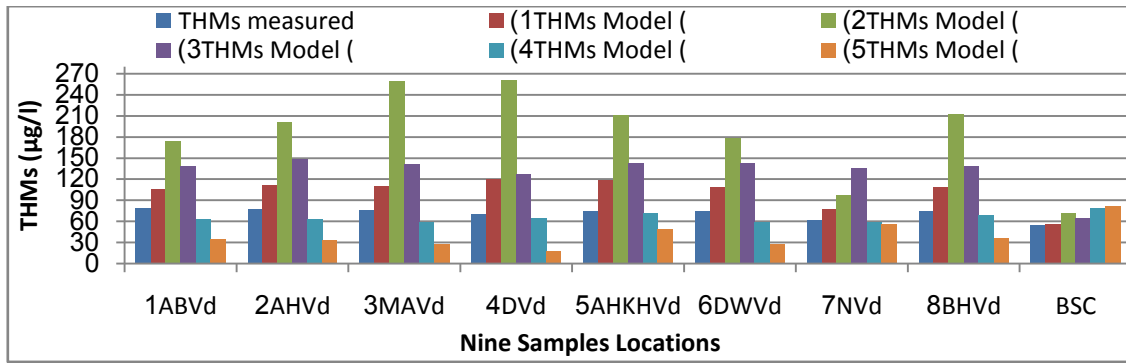
Figure 15. Averaged measured and predicted THMs by the five empirical models
