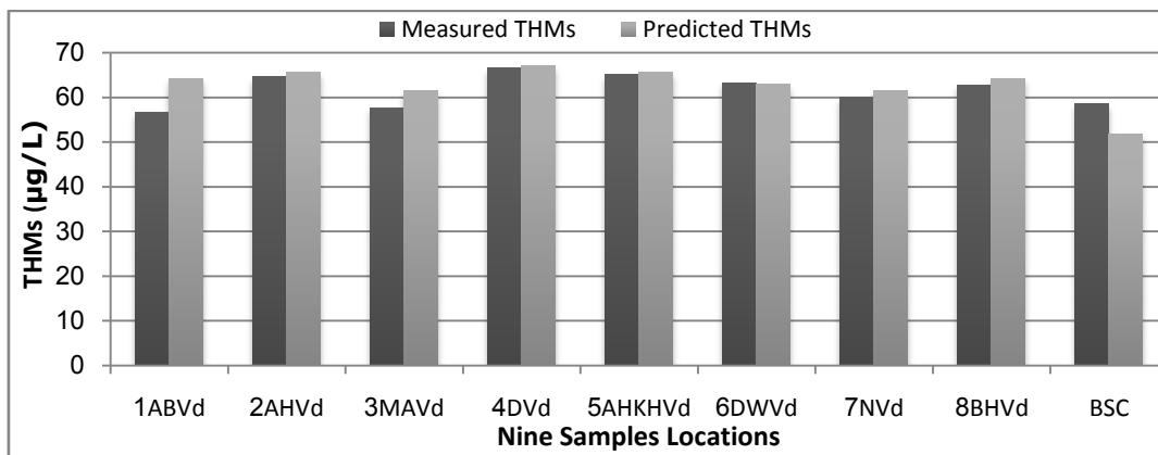
Figure 16. Averaged measured and predicted THMs by the model (6) at 8 / 6 / 2015
