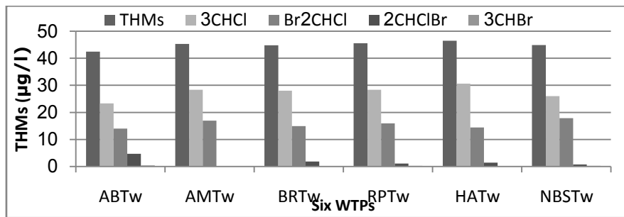
Figure 13. Averaged measured THMs with its components (µg/L) at the six WTPs
