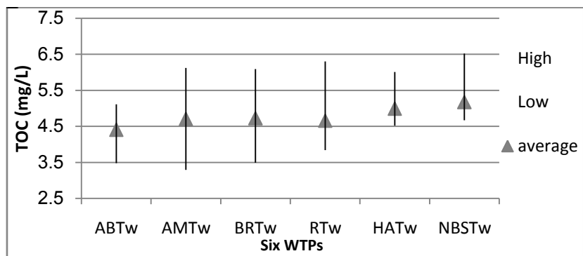
Figure 6. Concentrations of TOC at the exit of WTPs on BSWDN
