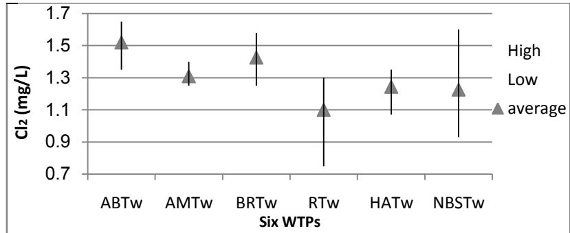
Figure 5. Concentrations of free residual chlorine at the exit of WTPs on BSWDN
