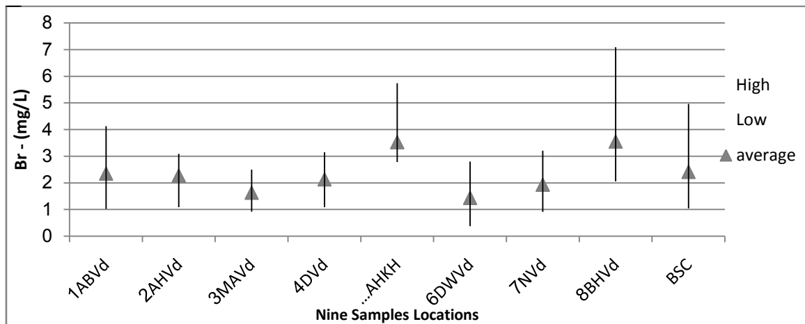
Figure 10. Concentrations of free bromide ion at the nine points on BSWDN
