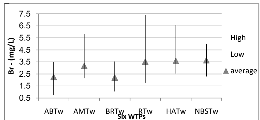
Figure 7. Concentrations of free bromide ion at the exit of WTPs on BSWDN
