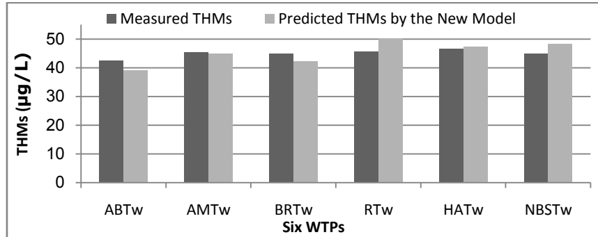
Figure 18. Averaged measured and predicted THMs by new Developed model
