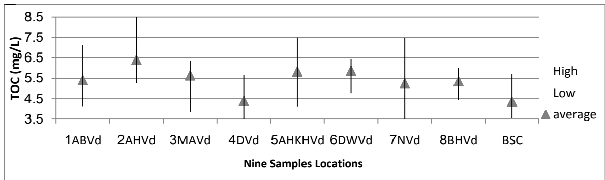
Figure 9. Concentrations of TOC at the nine points on BSWDN
