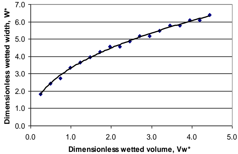
Fig. 2: Relationship between dimensionless variables W^* and V_w^* .
