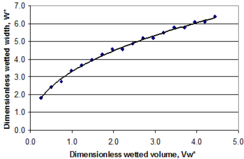
Fig. 1: Relationship between dimensionless variables W^* and V_w^* .
